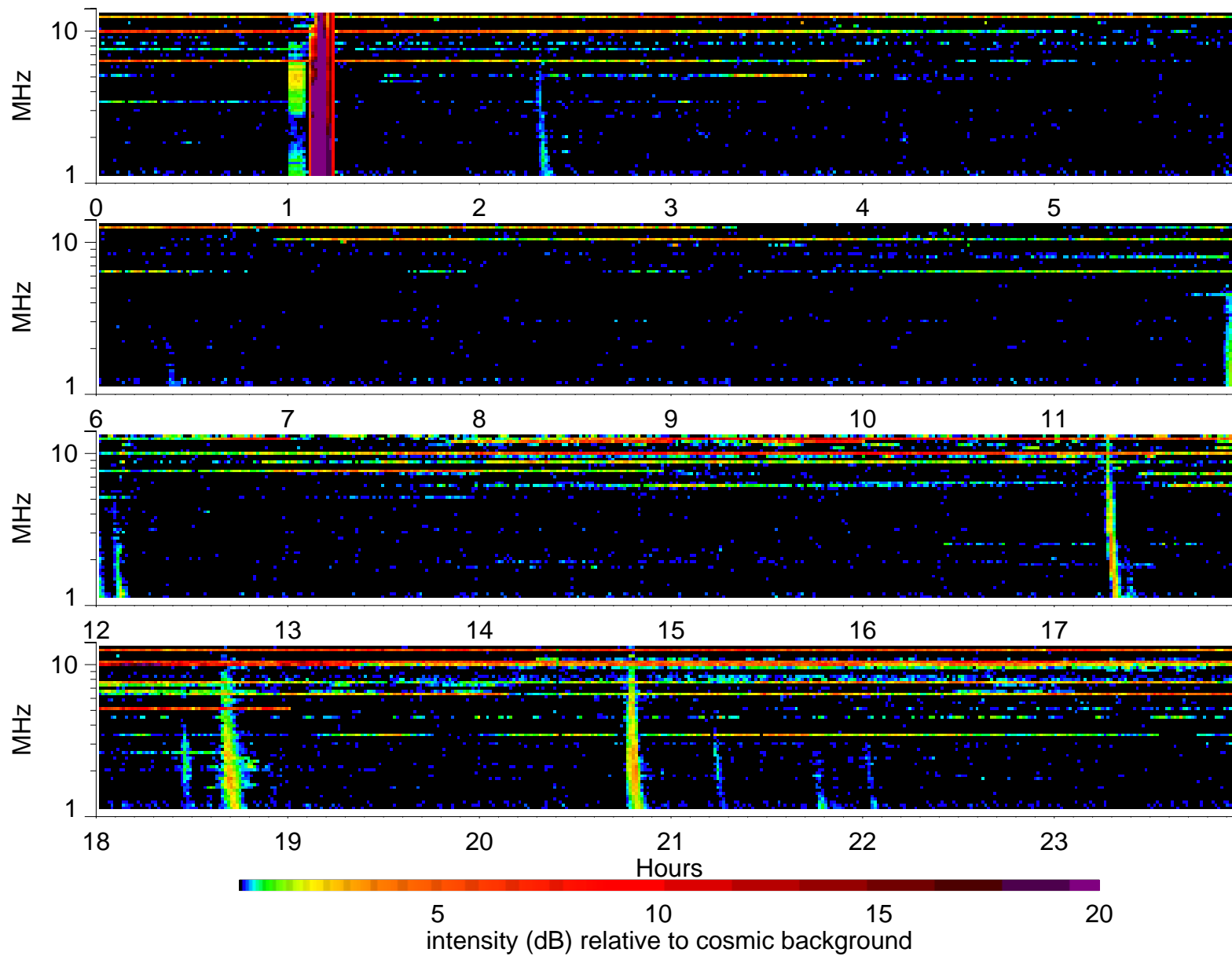
Wind Waves RAD2 receiver: 2003/8/14
