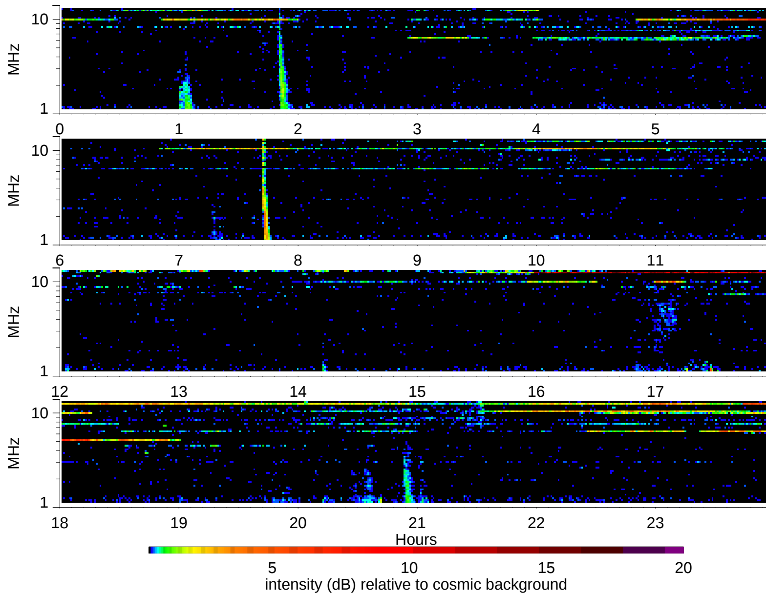
Wind Waves RAD2 receiver: 2003/8/9
