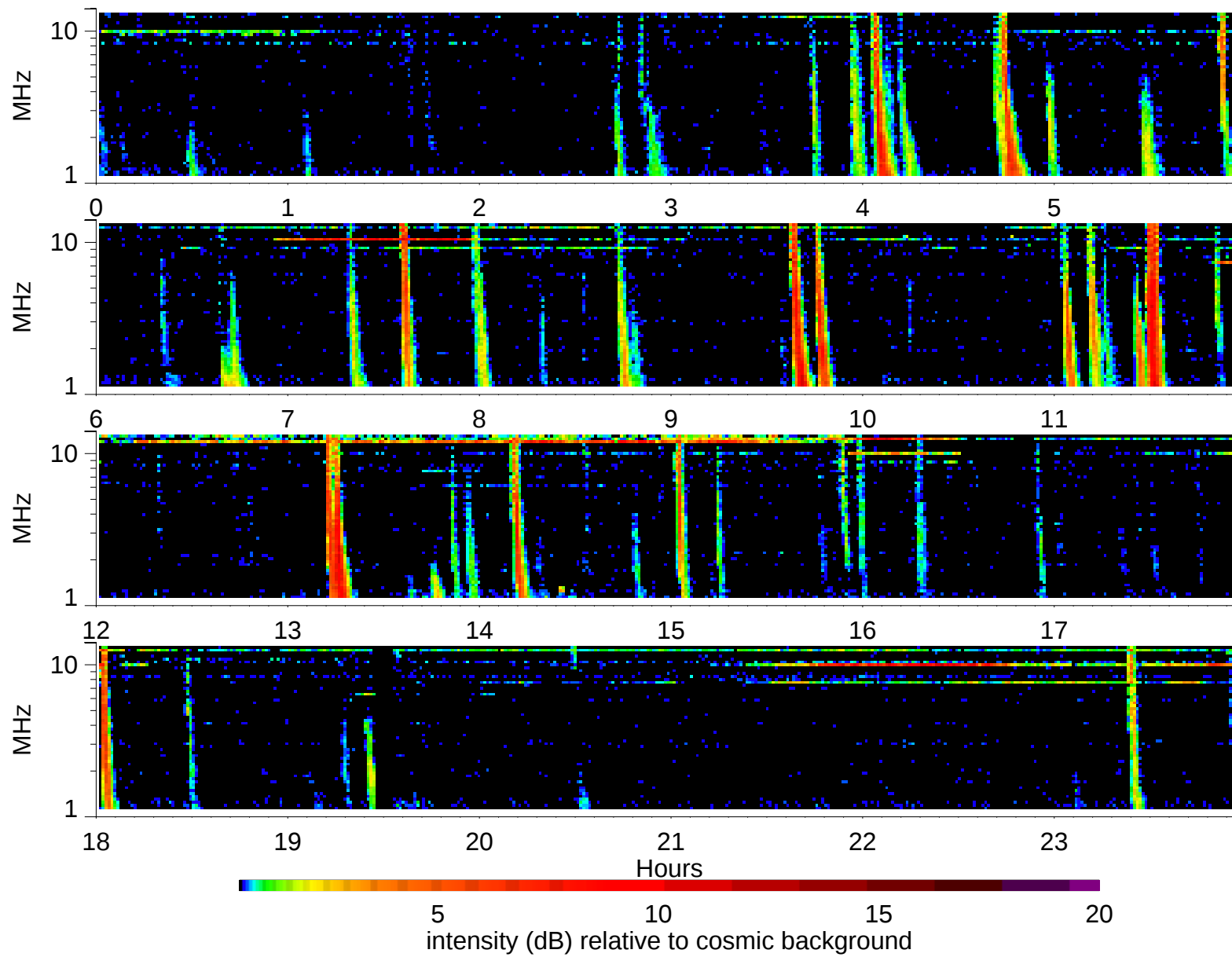
Wind Waves RAD2 receiver: 2003/8/7
