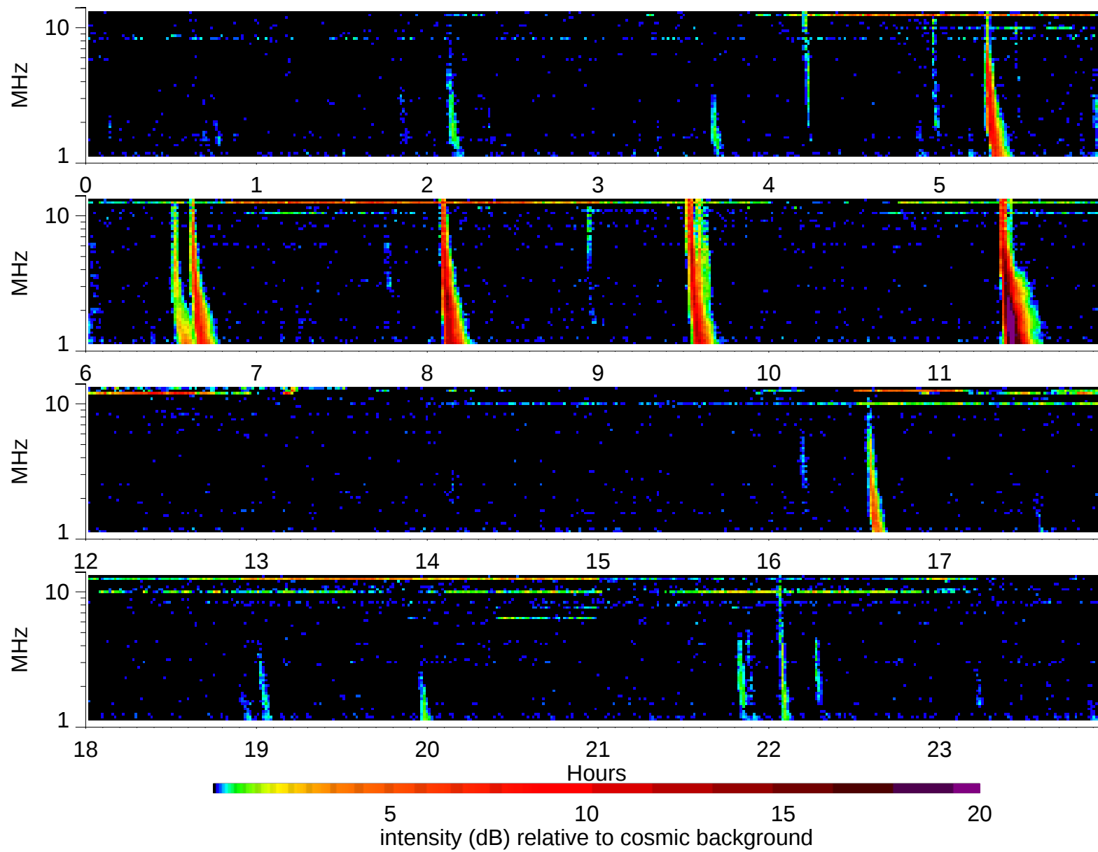
Wind Waves RAD2 receiver: 2003/8/5
