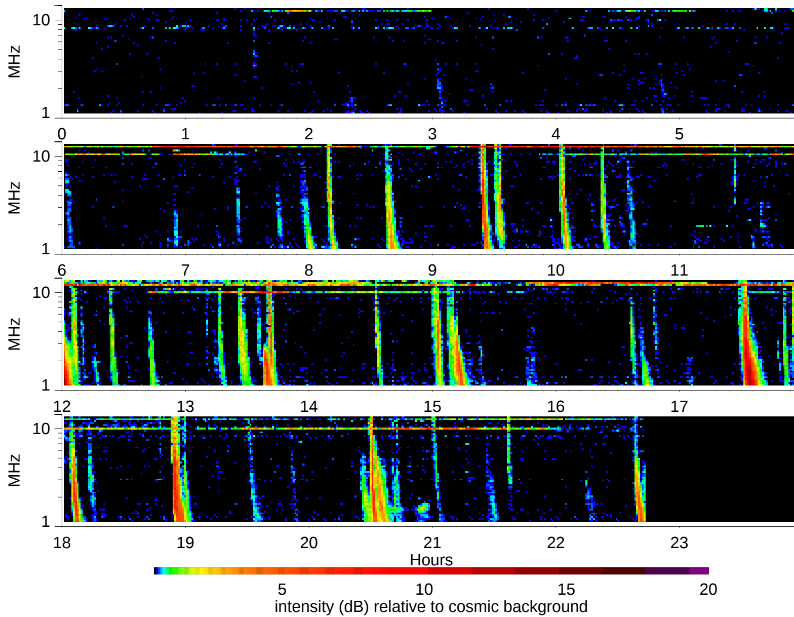
Wind Waves RAD2 receiver: 2003/8/3
