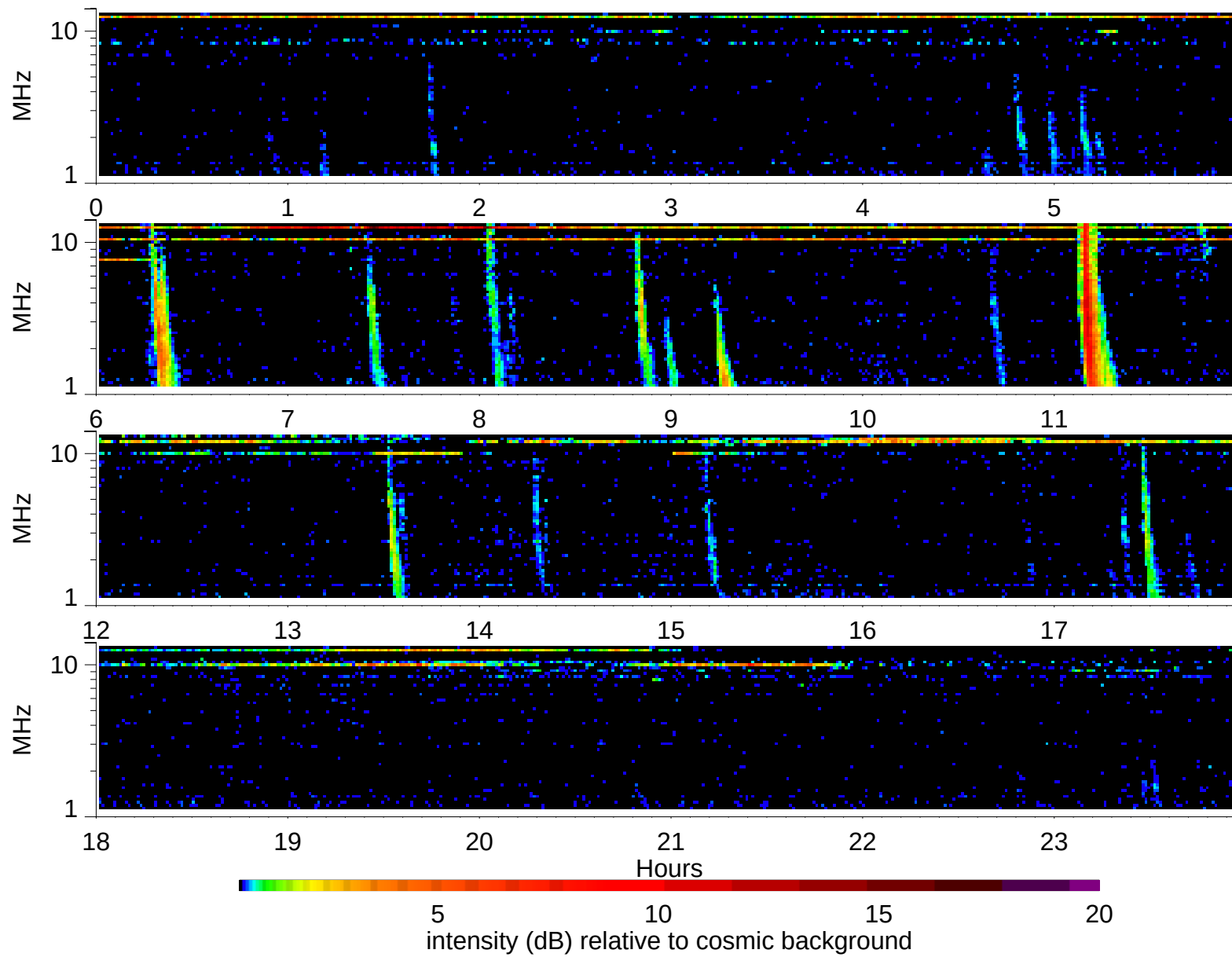
Wind Waves RAD2 receiver: 2003/7/28
