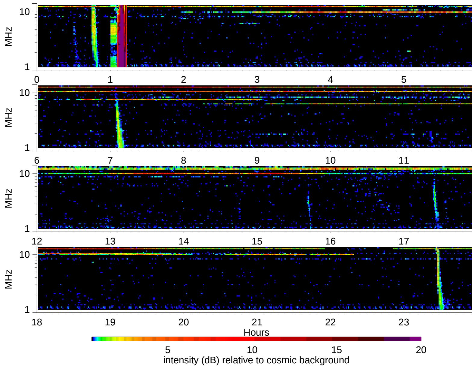
Wind Waves RAD2 receiver: 2003/7/27
