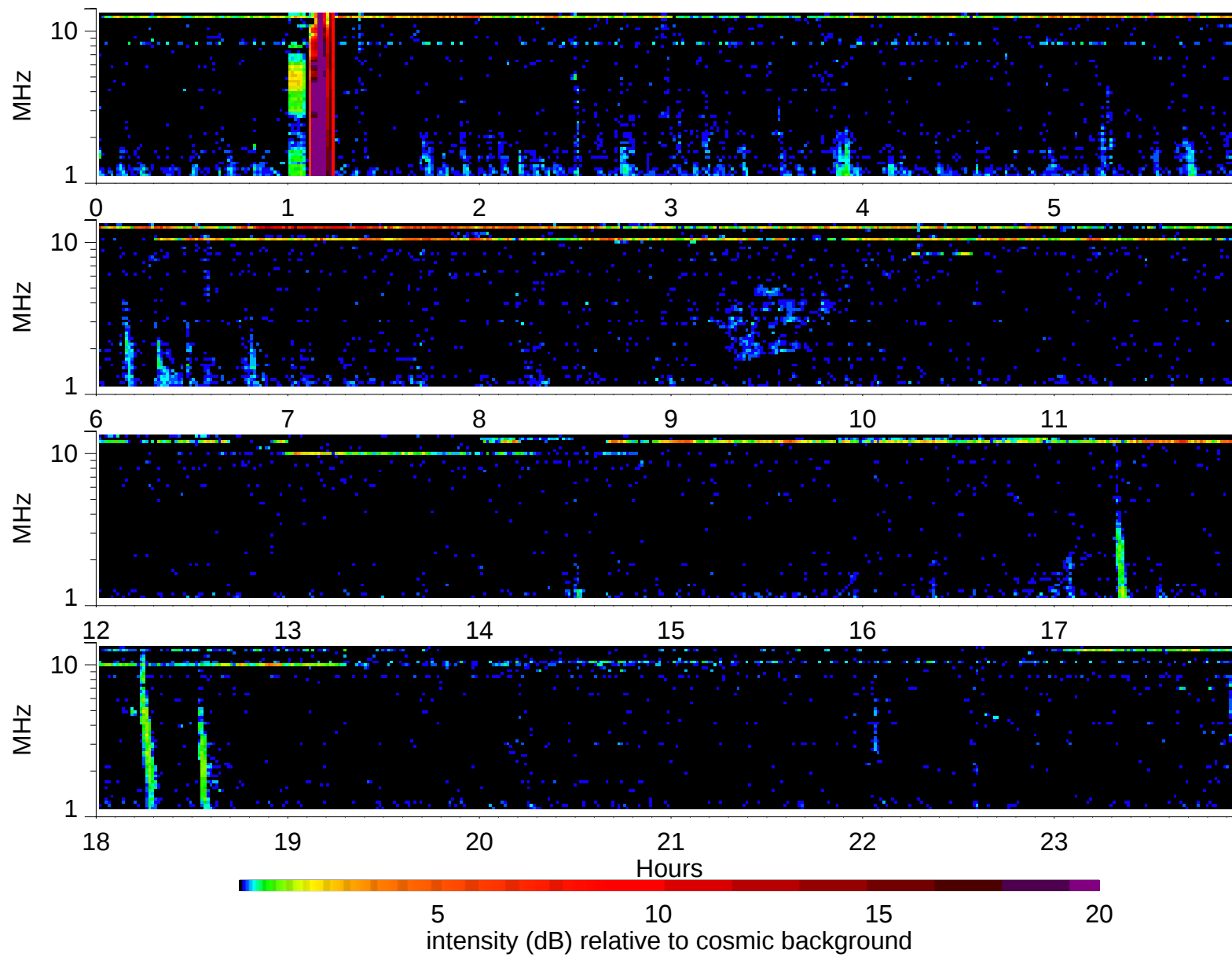
Wind Waves RAD2 receiver: 2003/7/23
