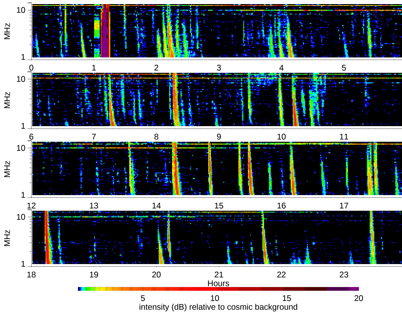
Wind Waves RAD2 receiver: 2003/7/21
