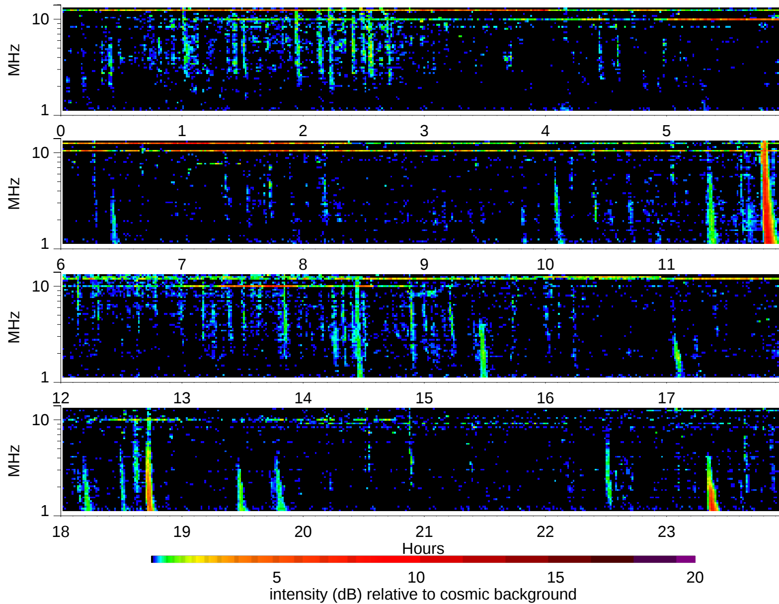
Wind Waves RAD2 receiver: 2003/7/20
