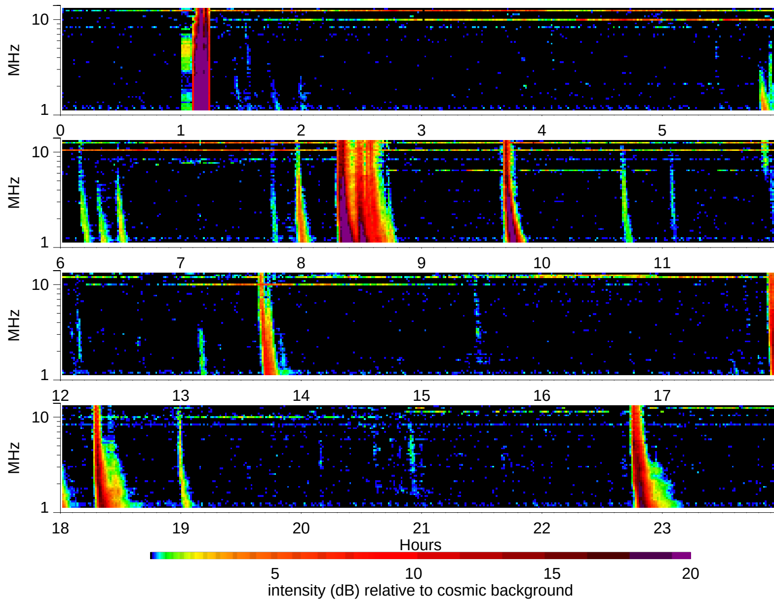
Wind Waves RAD2 receiver: 2003/7/17
