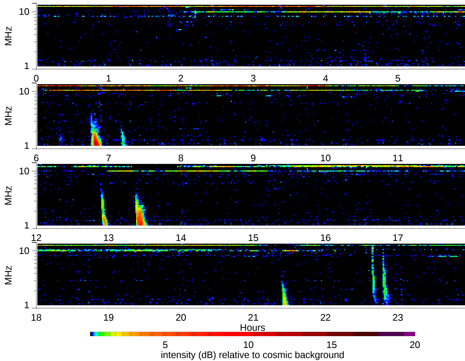
Wind Waves RAD2 receiver: 2003/7/16
