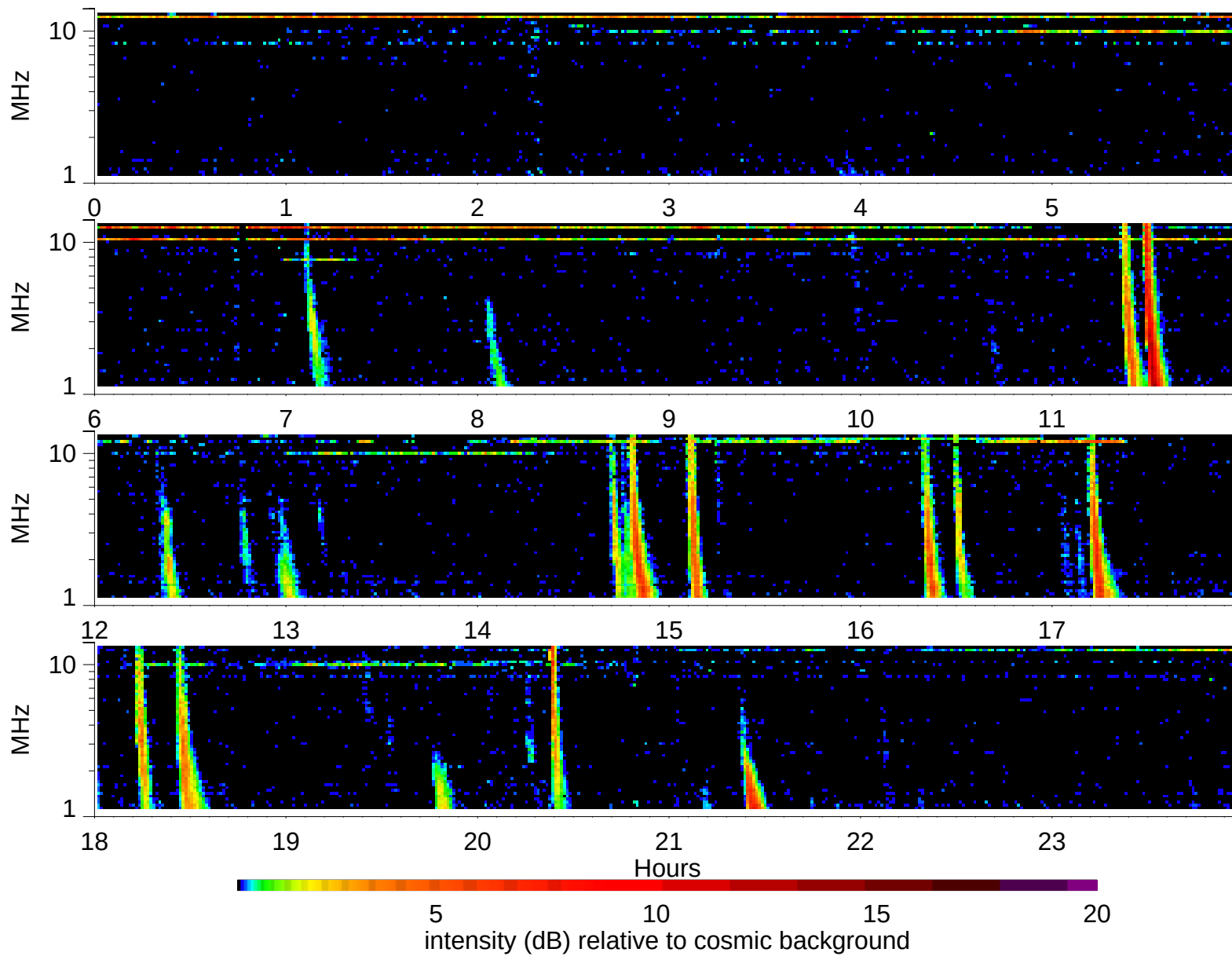
Wind Waves RAD2 receiver: 2003/7/14
