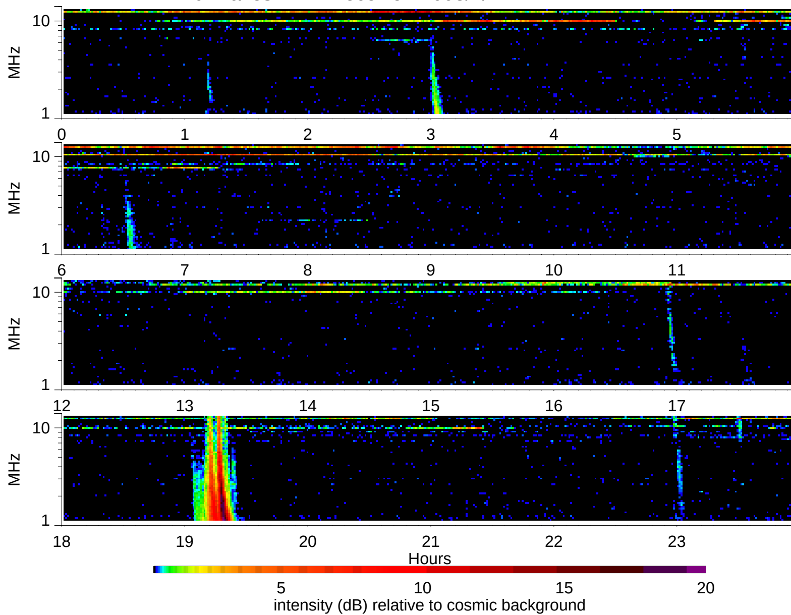
Wind Waves RAD2 receiver: 2003/7/12
