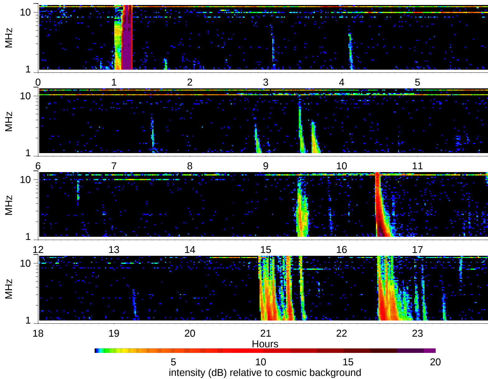
Wind Waves RAD2 receiver: 2003/7/9
