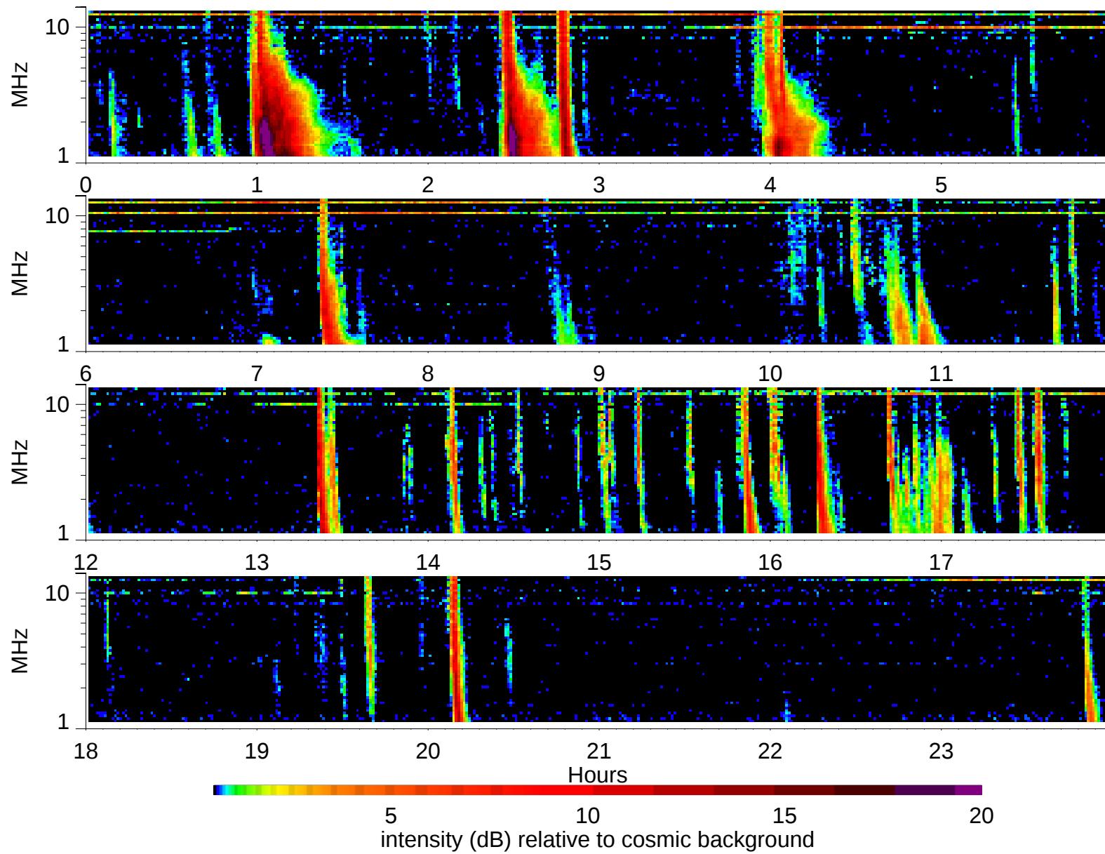
Wind Waves RAD2 receiver: 2003/7/8
