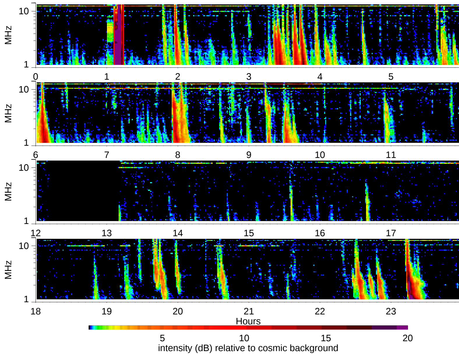
Wind Waves RAD2 receiver: 2003/7/7
