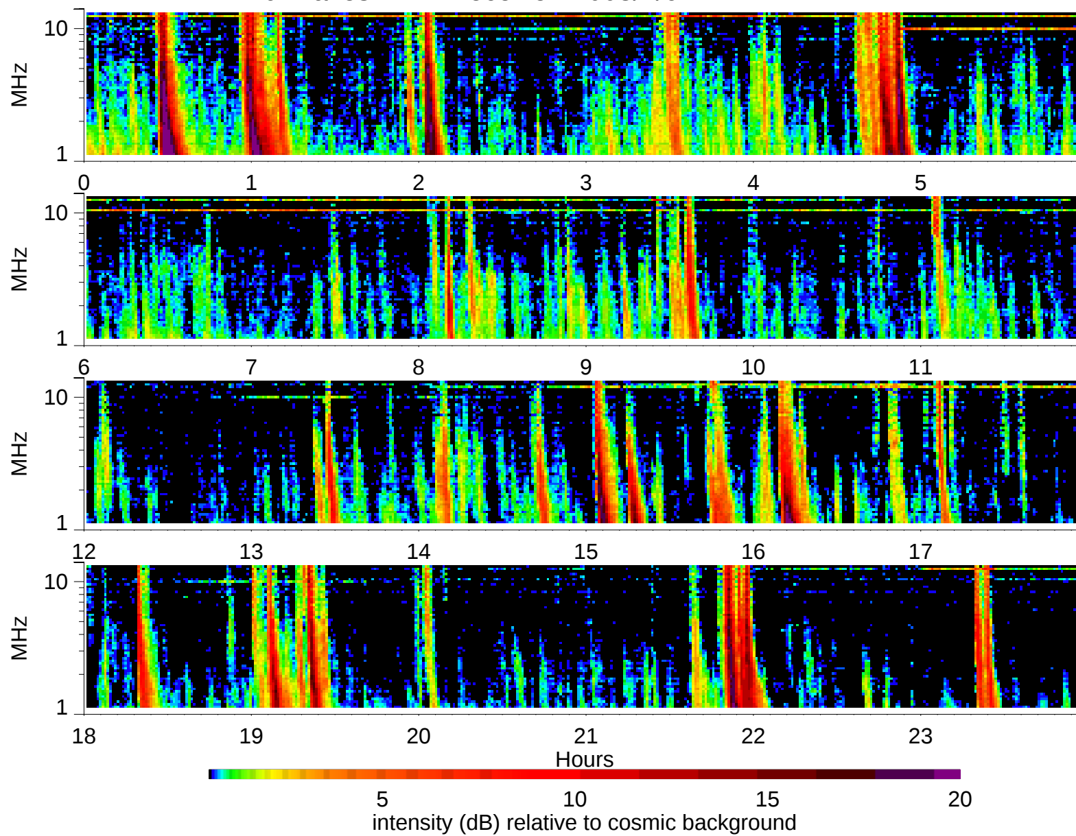
Wind Waves RAD2 receiver: 2003/7/6
