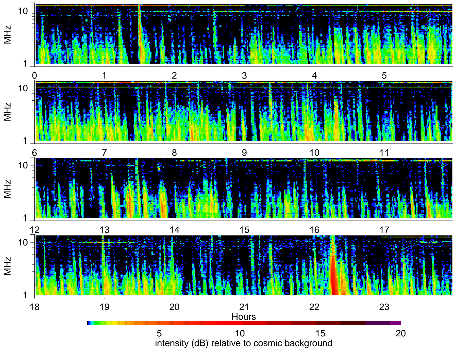
Wind Waves RAD2 receiver: 2003/7/2
