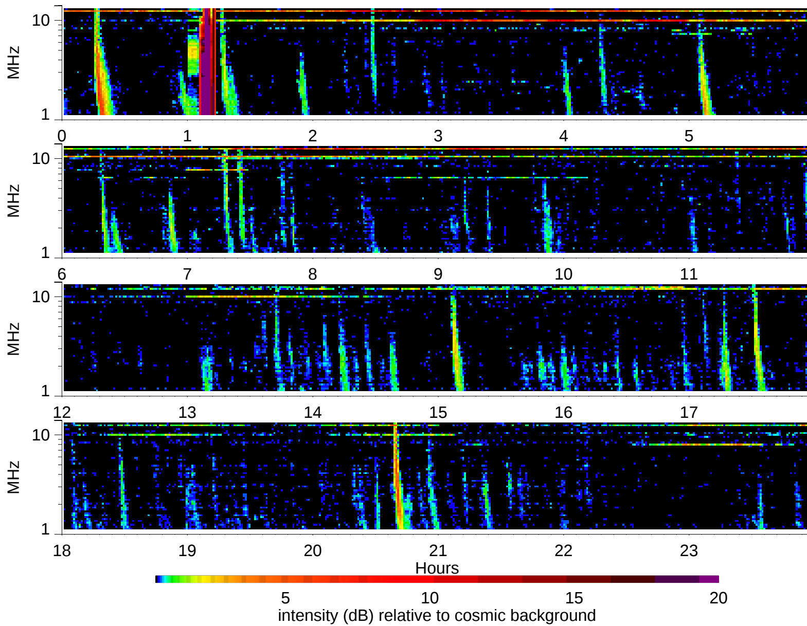
Wind Waves RAD2 receiver: 2003/6/27
