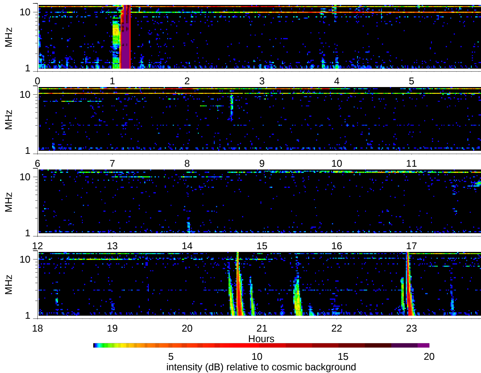
Wind Waves RAD2 receiver: 2003/6/23
