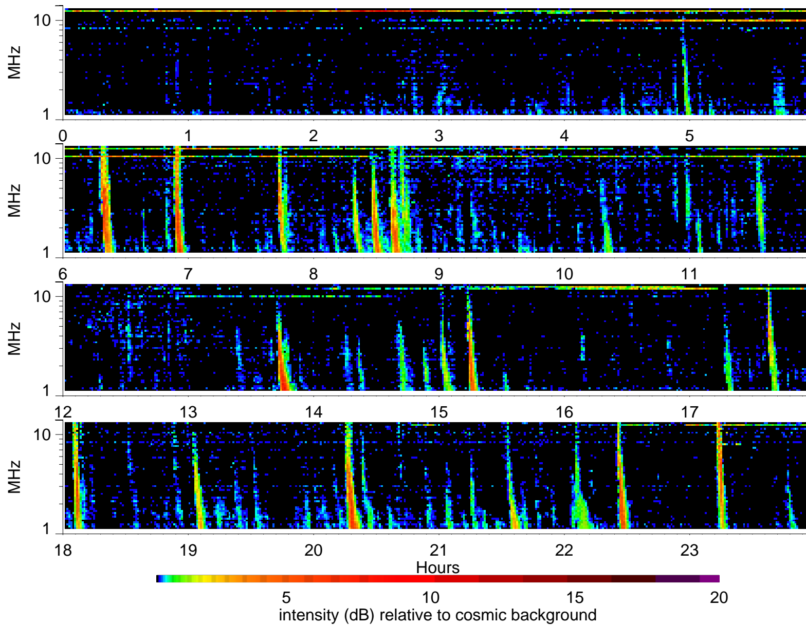
Wind Waves RAD2 receiver: 2003/6/20
