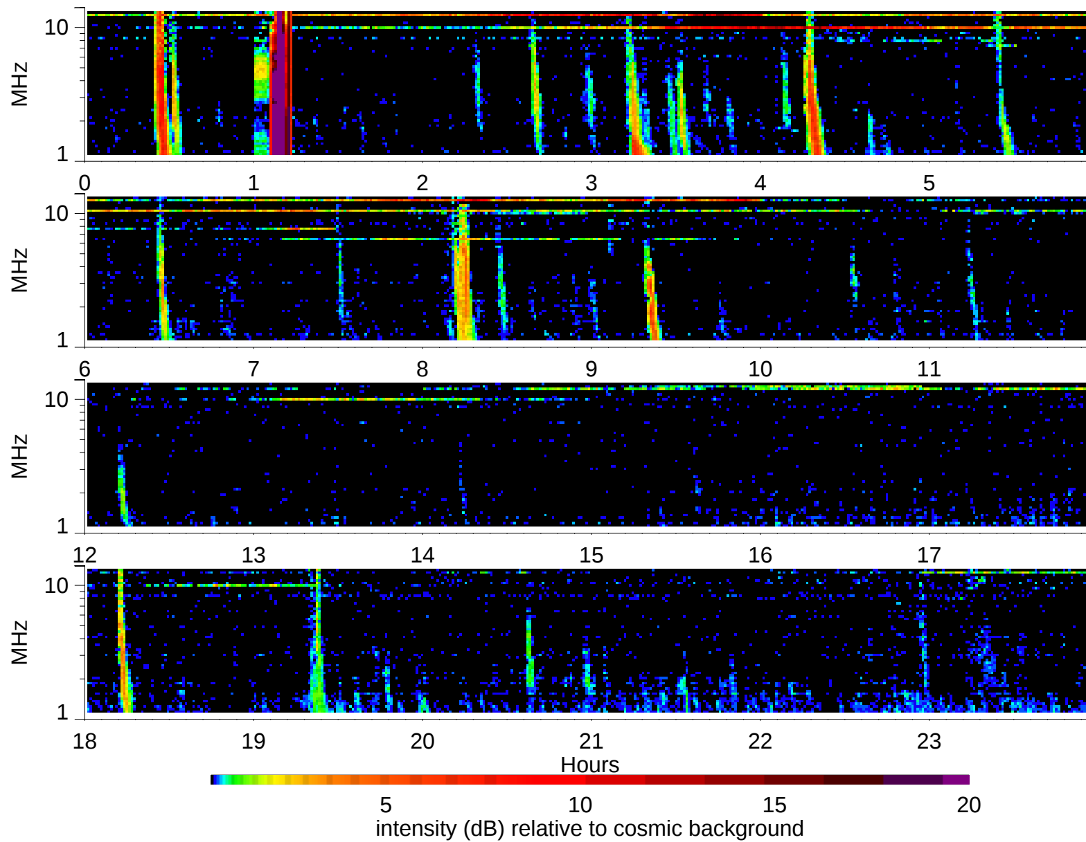
Wind Waves RAD2 receiver: 2003/6/19
