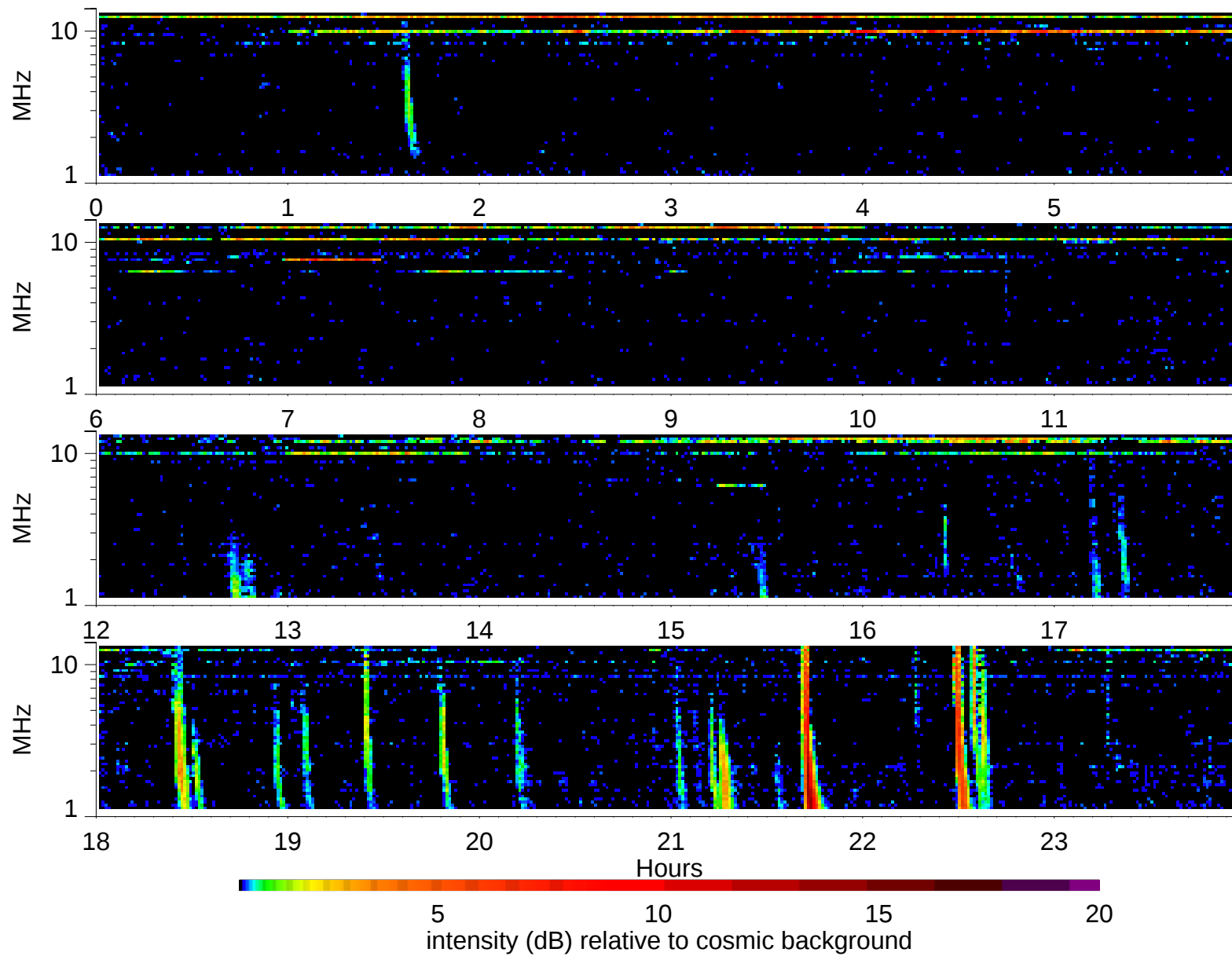
Wind Waves RAD2 receiver: 2003/6/18
