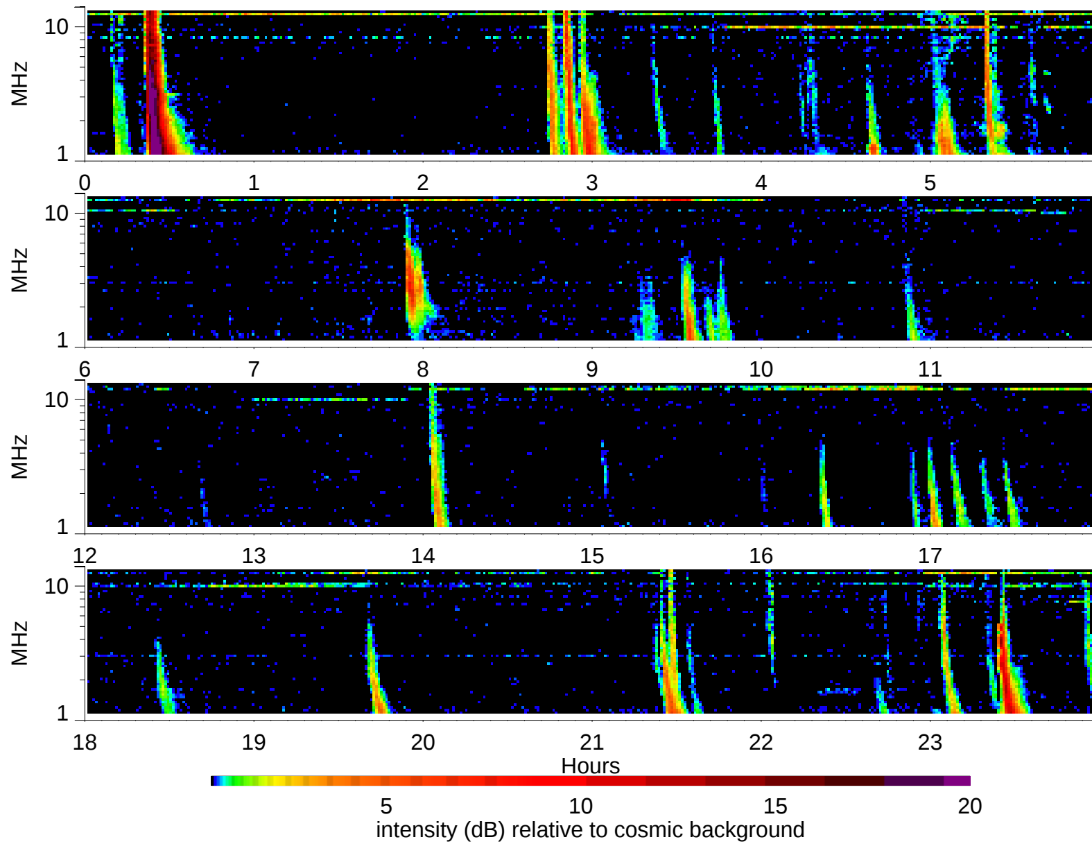
Wind Waves RAD2 receiver: 2003/6/14
