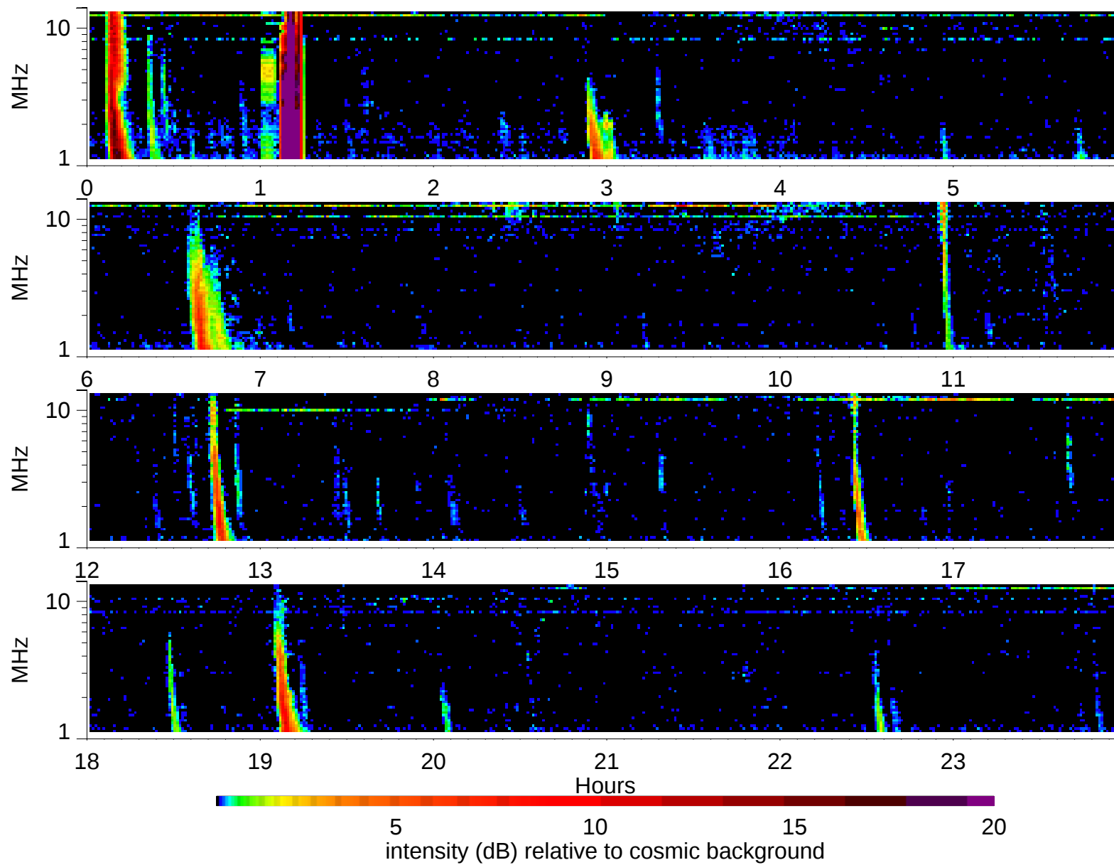
Wind Waves RAD2 receiver: 2003/6/13
