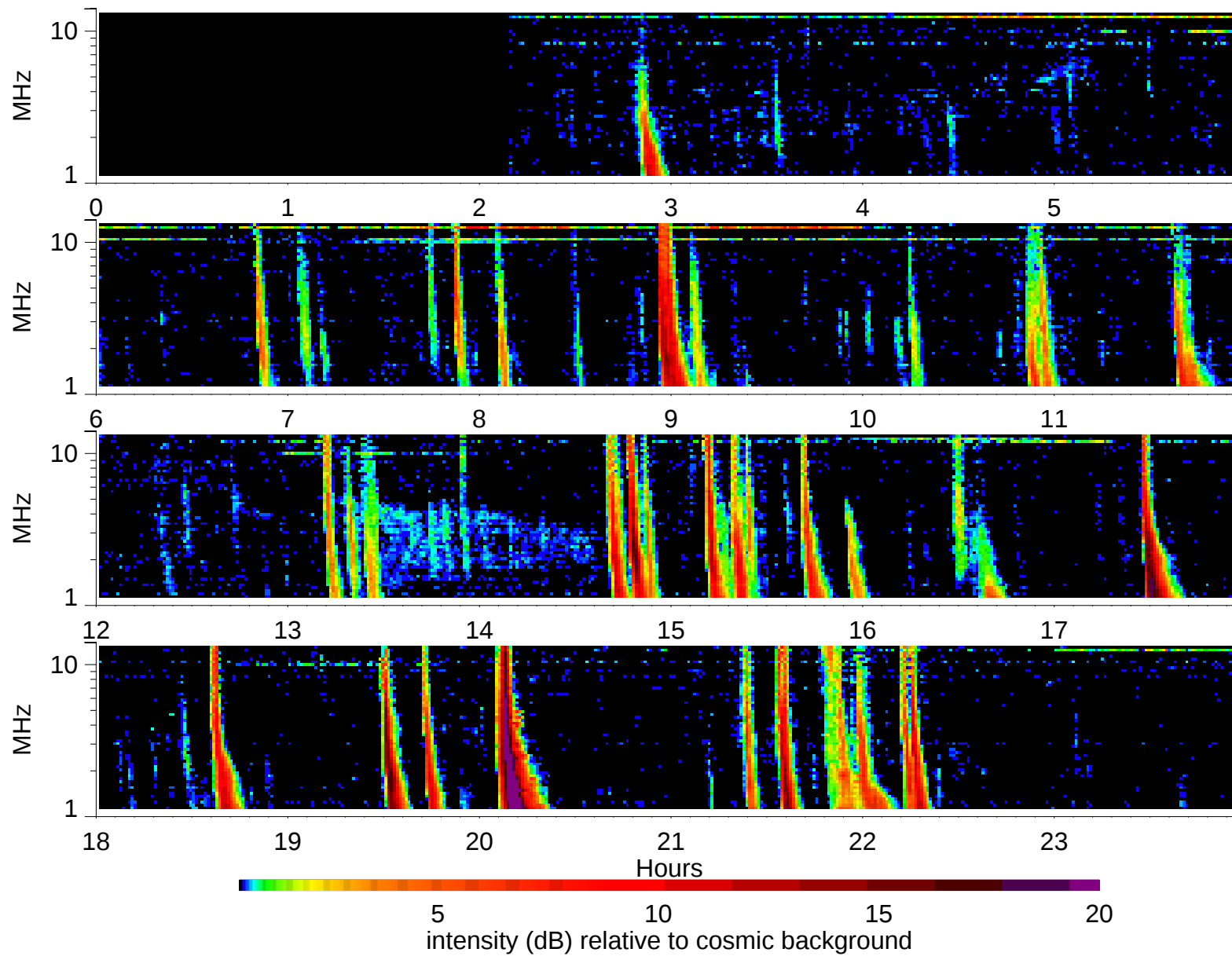
Wind Waves RAD2 receiver: 2003/6/11
