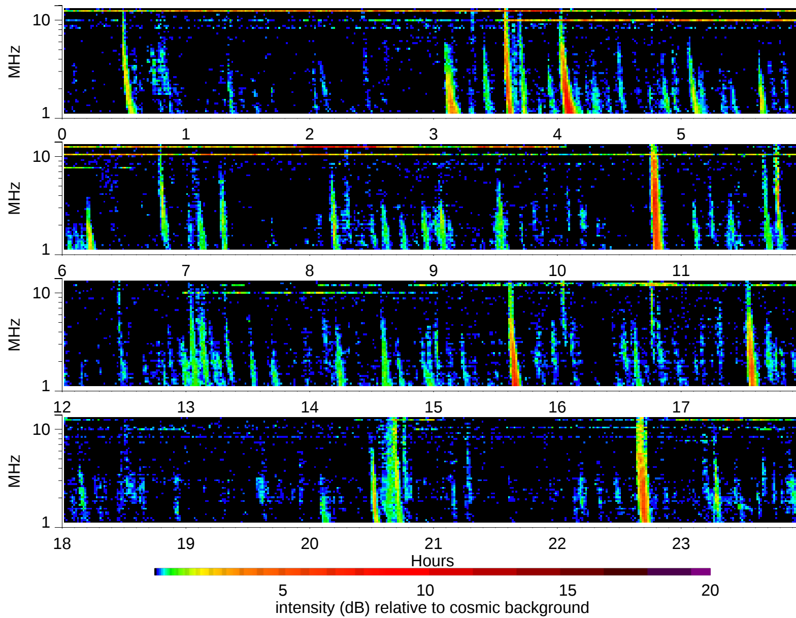
Wind Waves RAD2 receiver: 2003/6/8
