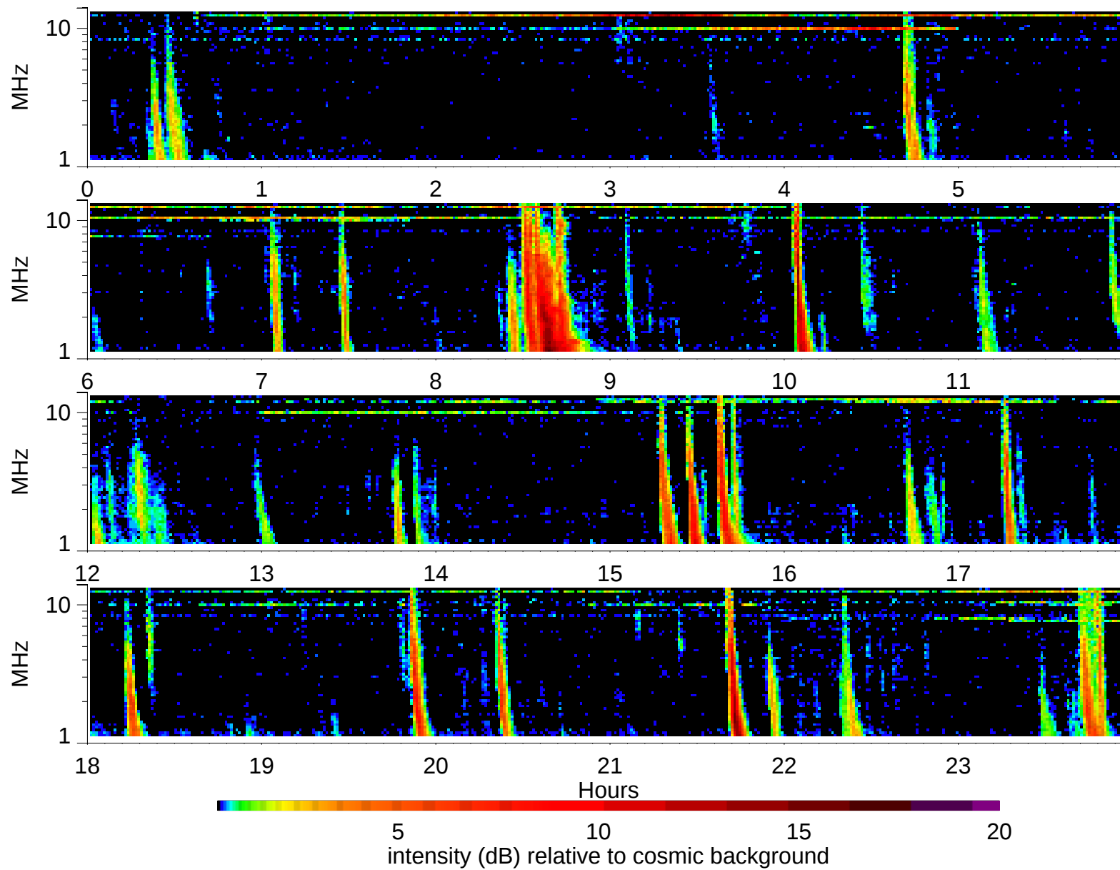
Wind Waves RAD2 receiver: 2003/6/2
