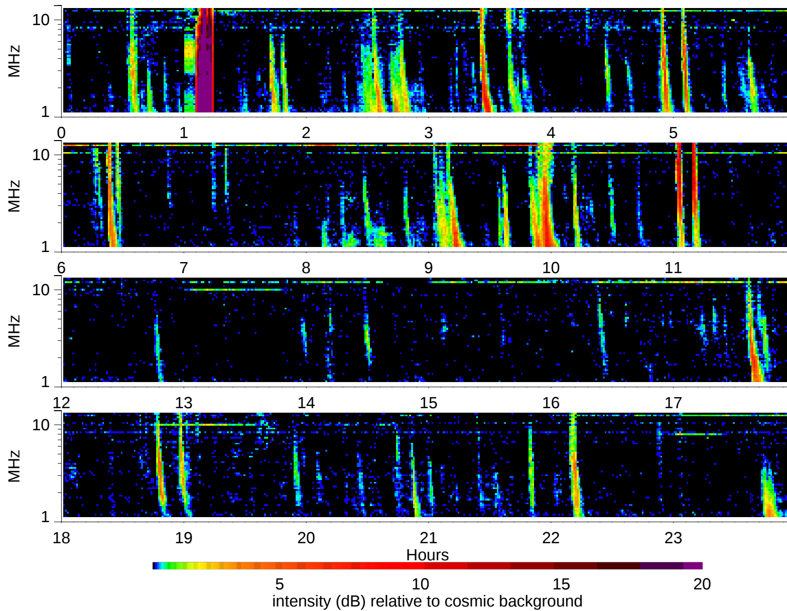
Wind Waves RAD2 receiver: 2003/6/1
