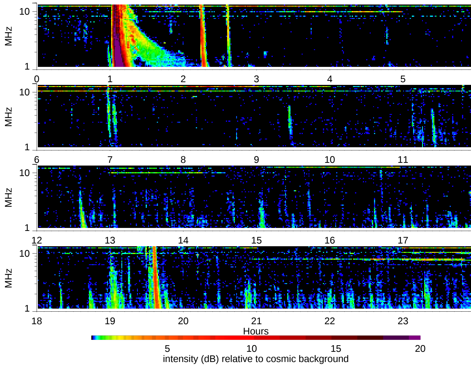
Wind Waves RAD2 receiver: 2003/5/29
