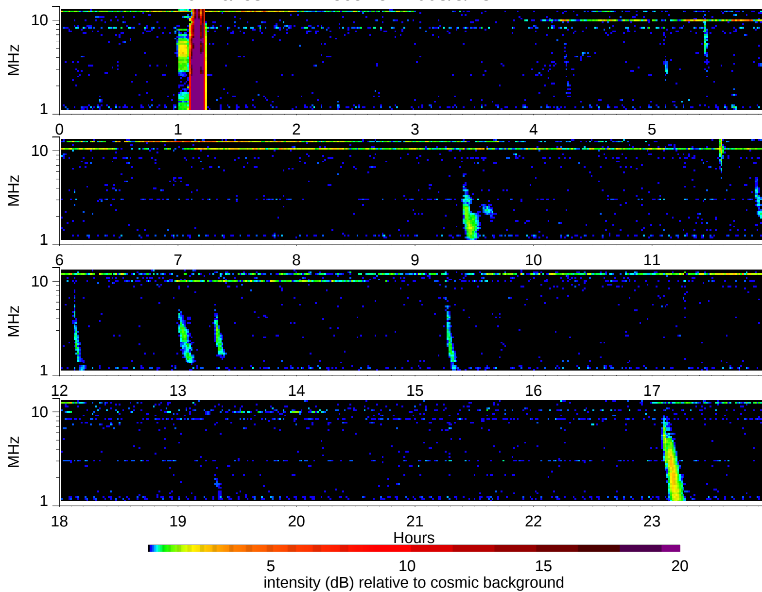
Wind Waves RAD2 receiver: 2003/5/18
