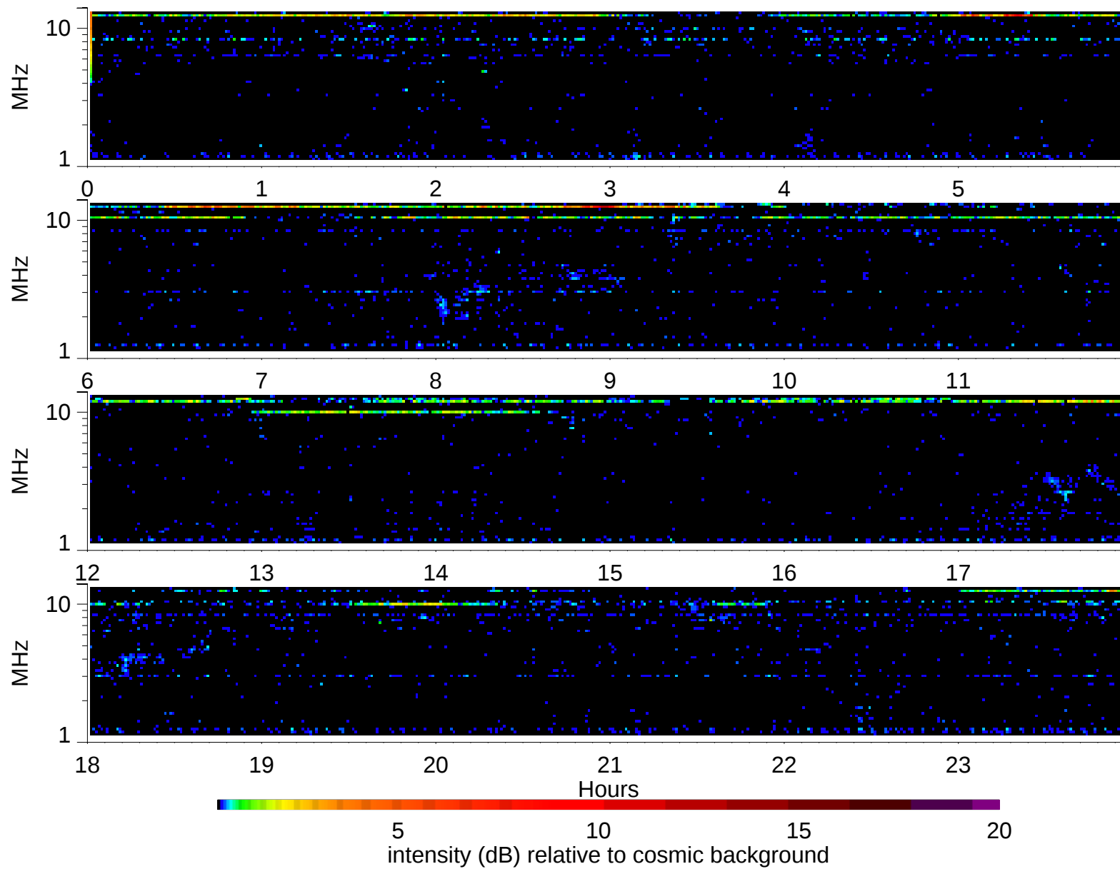
Wind Waves RAD2 receiver: 2003/5/15
