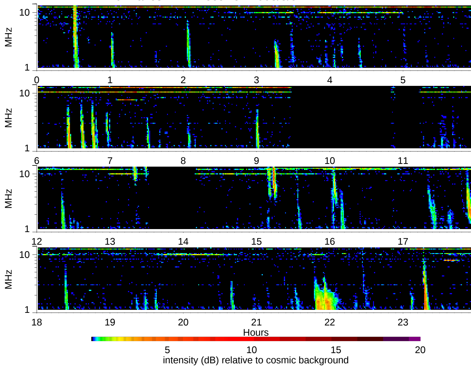
Wind Waves RAD2 receiver: 2003/5/9
