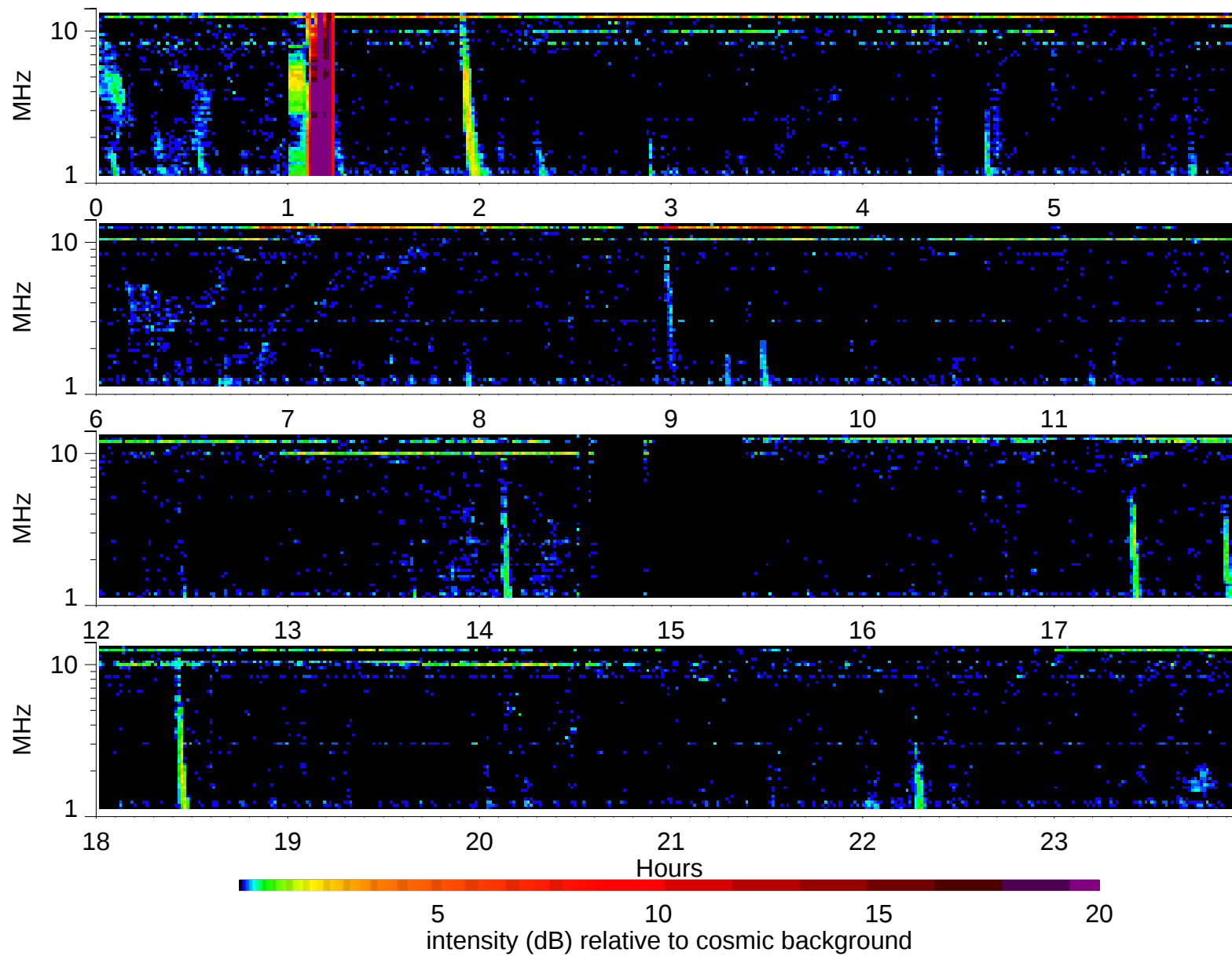
Wind Waves RAD2 receiver: 2003/5/8
