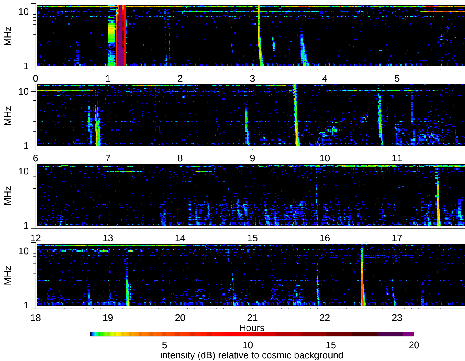
Wind Waves RAD2 receiver: 2003/5/6
