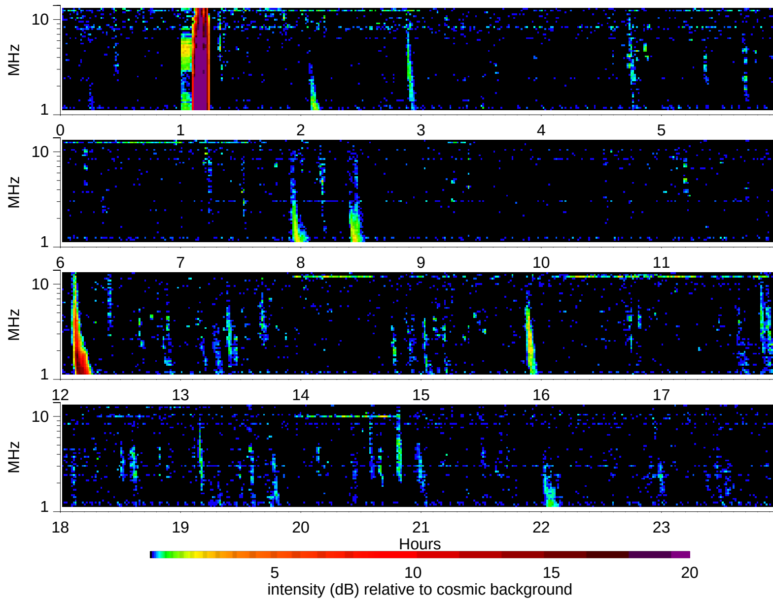
Wind Waves RAD2 receiver: 2003/5/2
