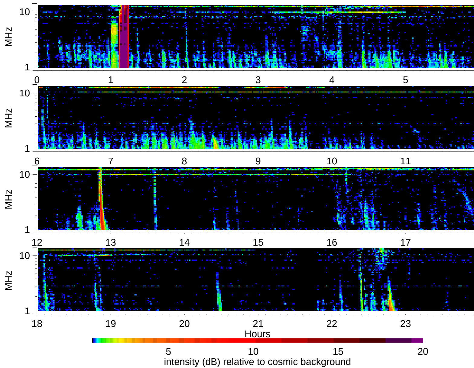
Wind Waves RAD2 receiver: 2003/4/30
