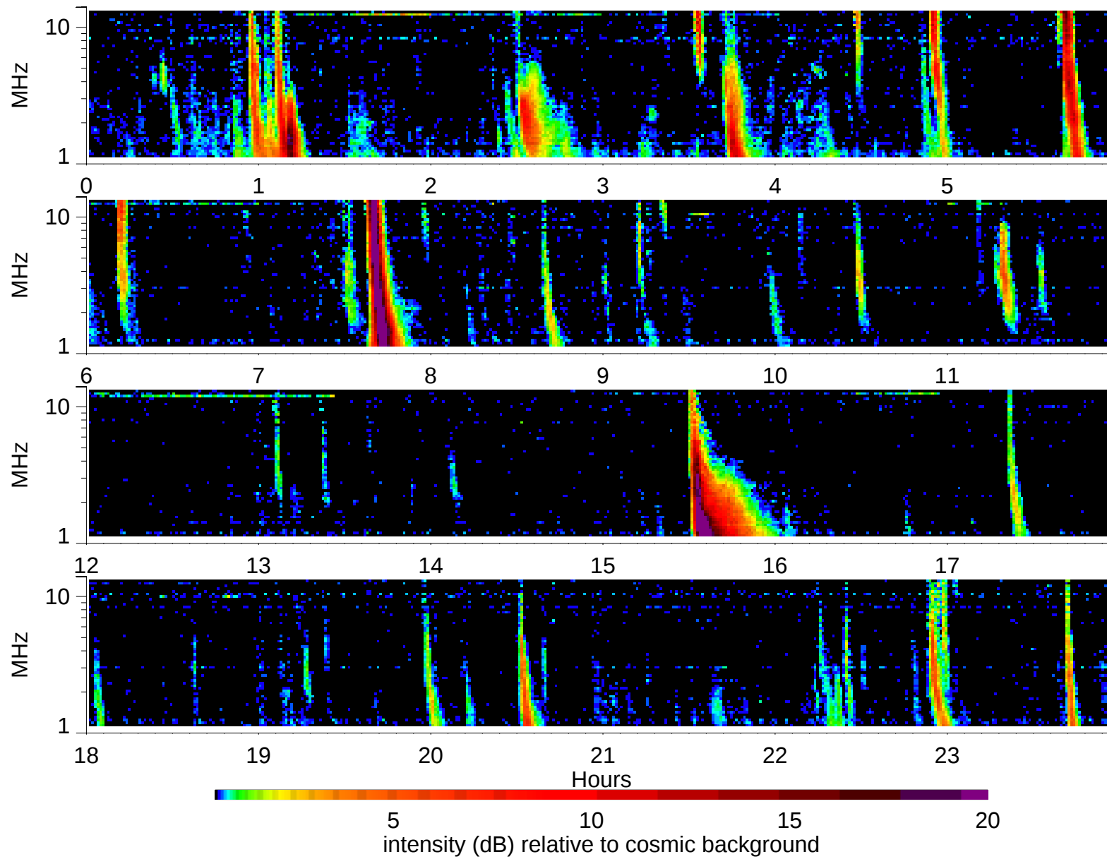
Wind Waves RAD2 receiver: 2003/4/27
