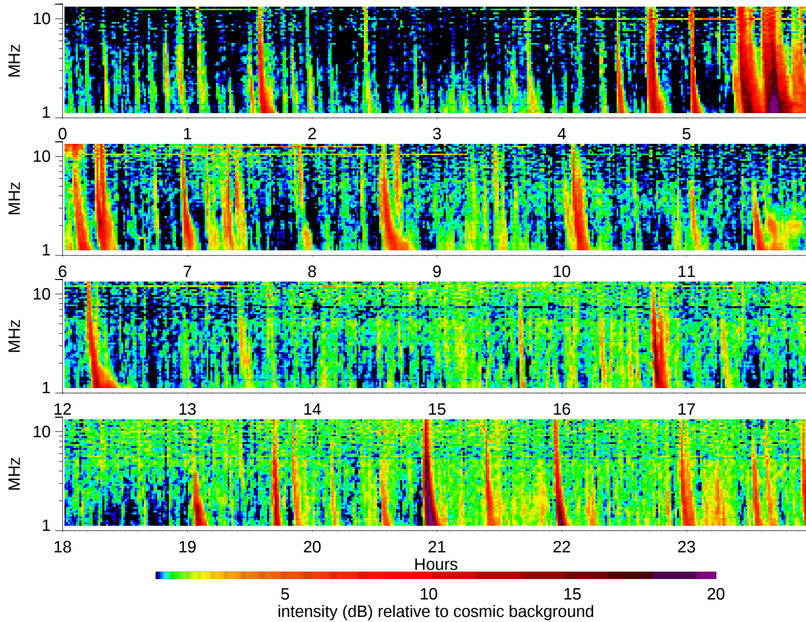
Wind Waves RAD2 receiver: 2003/4/25
