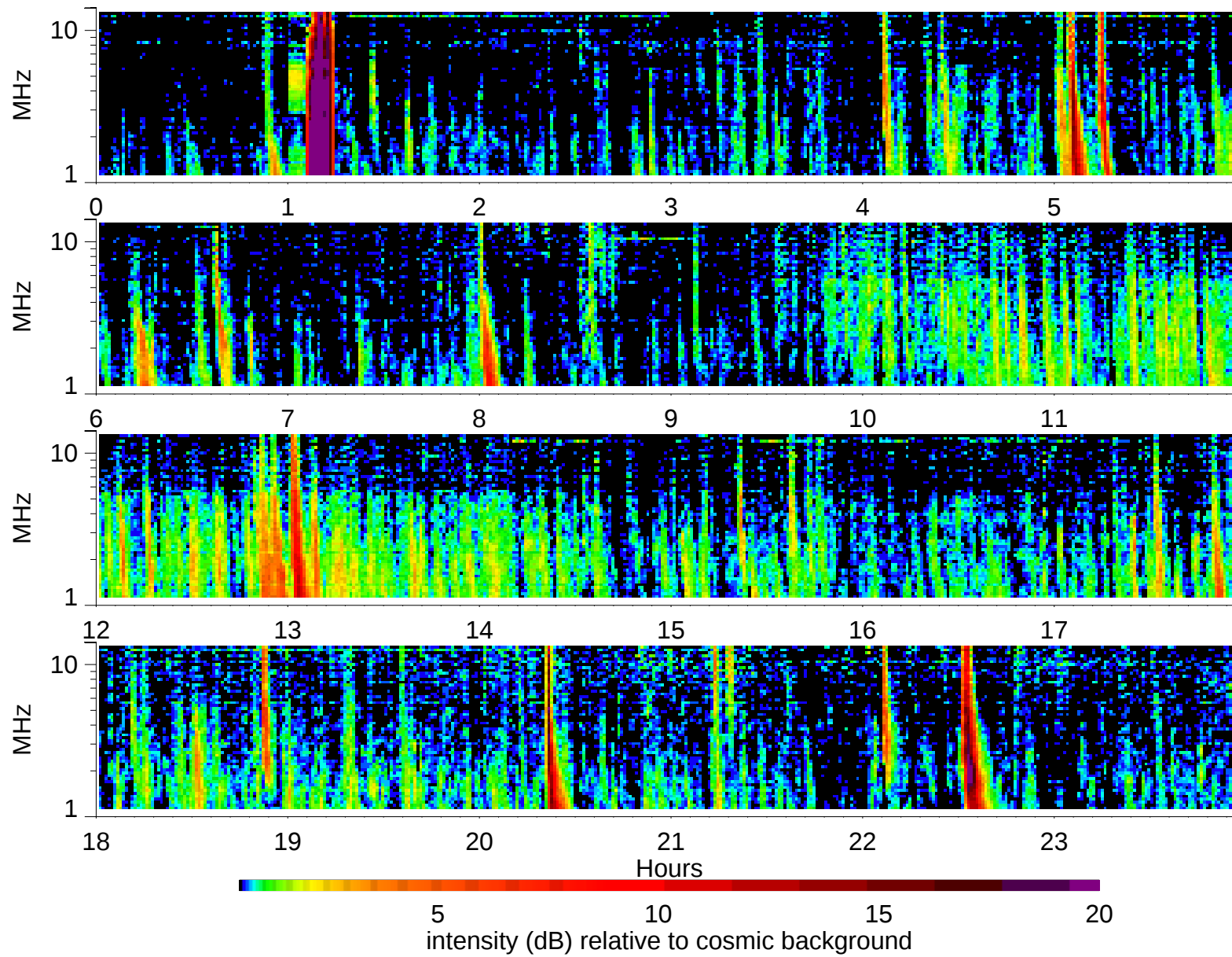
Wind Waves RAD2 receiver: 2003/4/24
