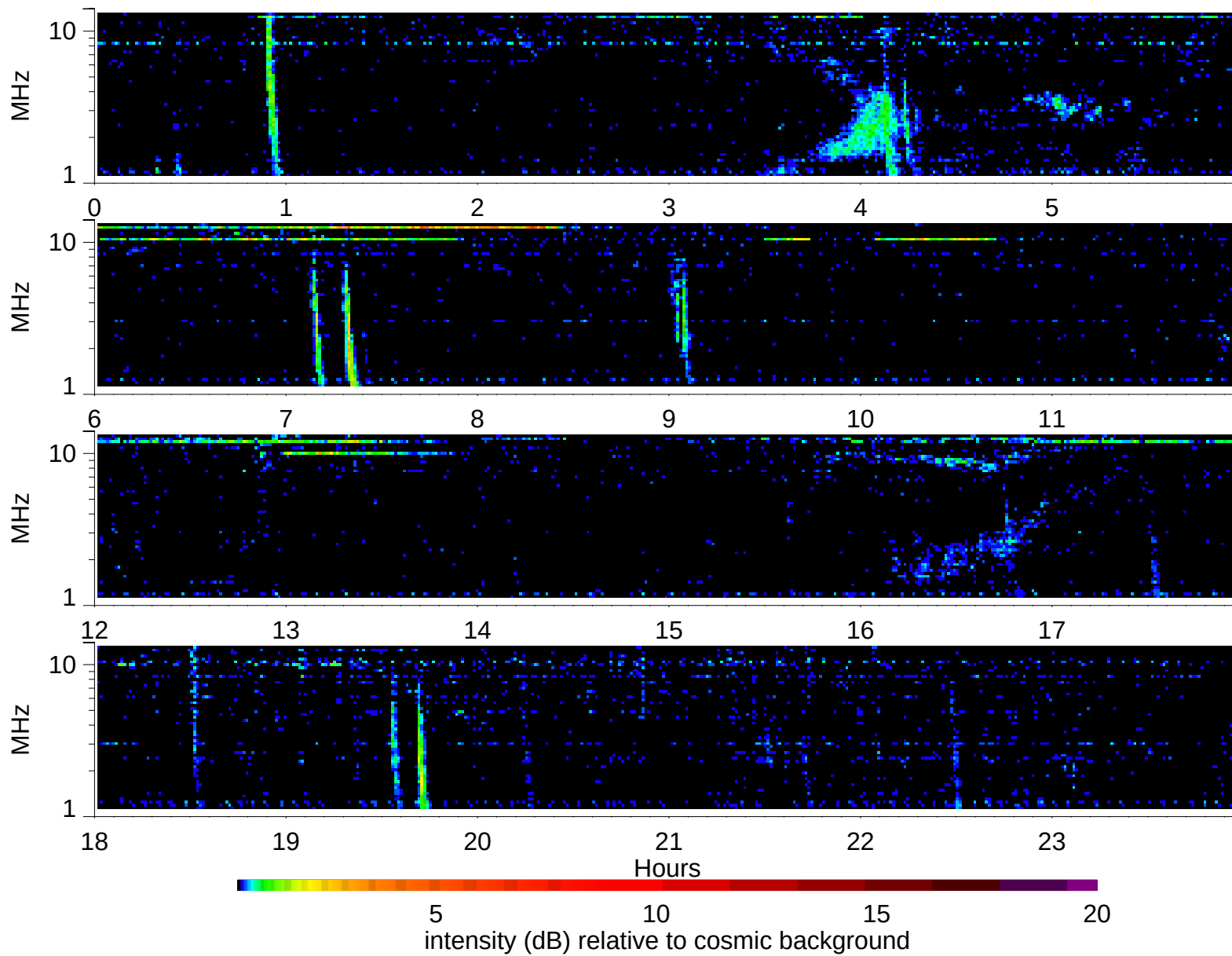
Wind Waves RAD2 receiver: 2003/4/19
