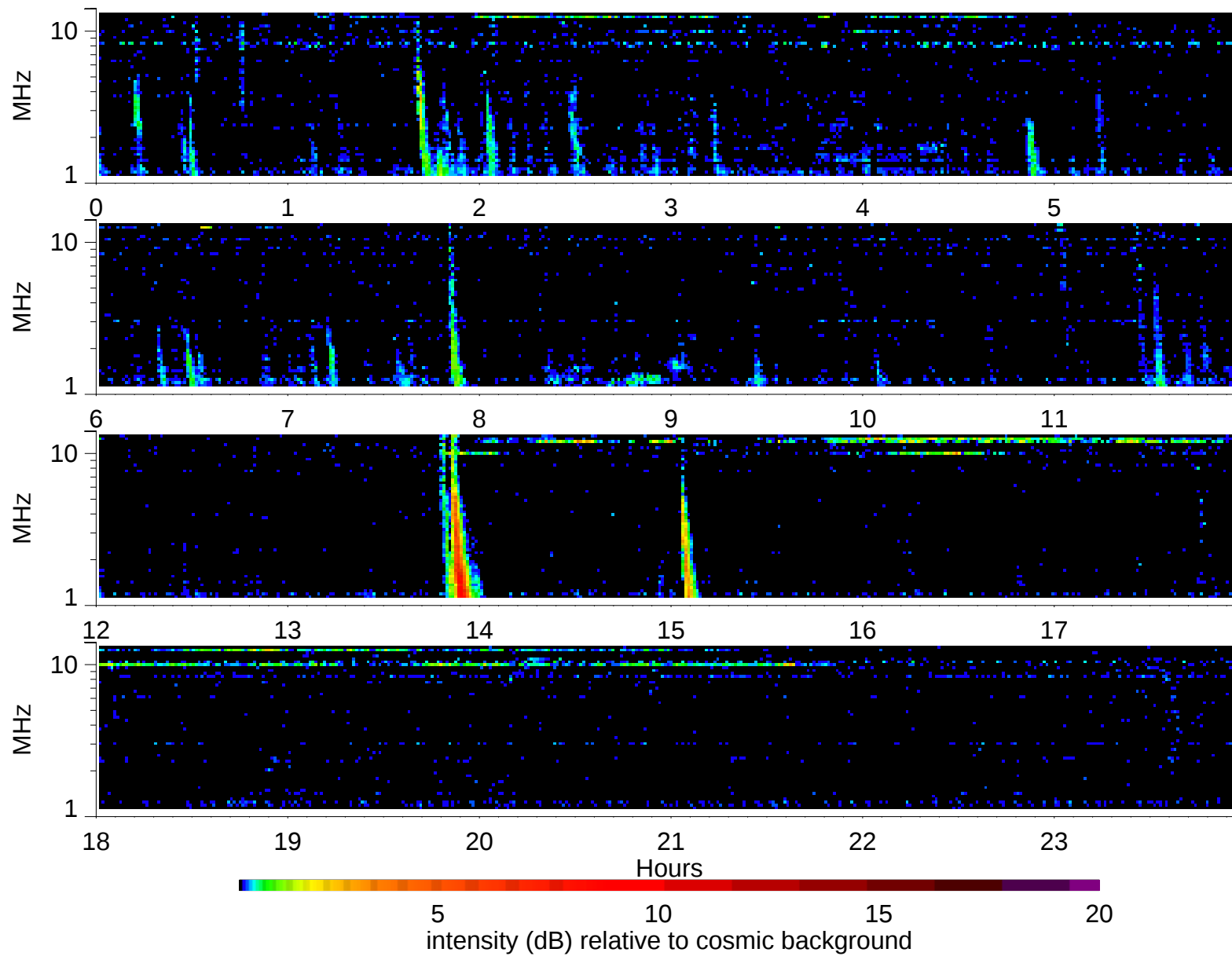
Wind Waves RAD2 receiver: 2003/4/15
