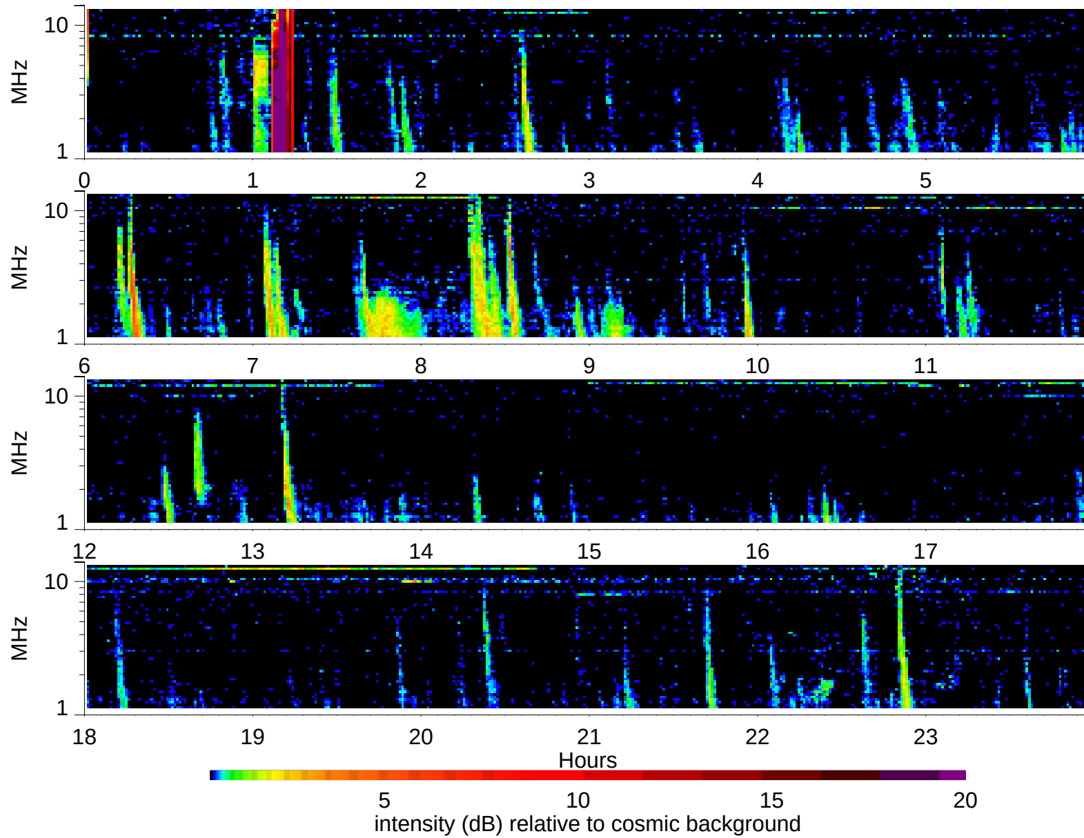
Wind Waves RAD2 receiver: 2003/4/14
