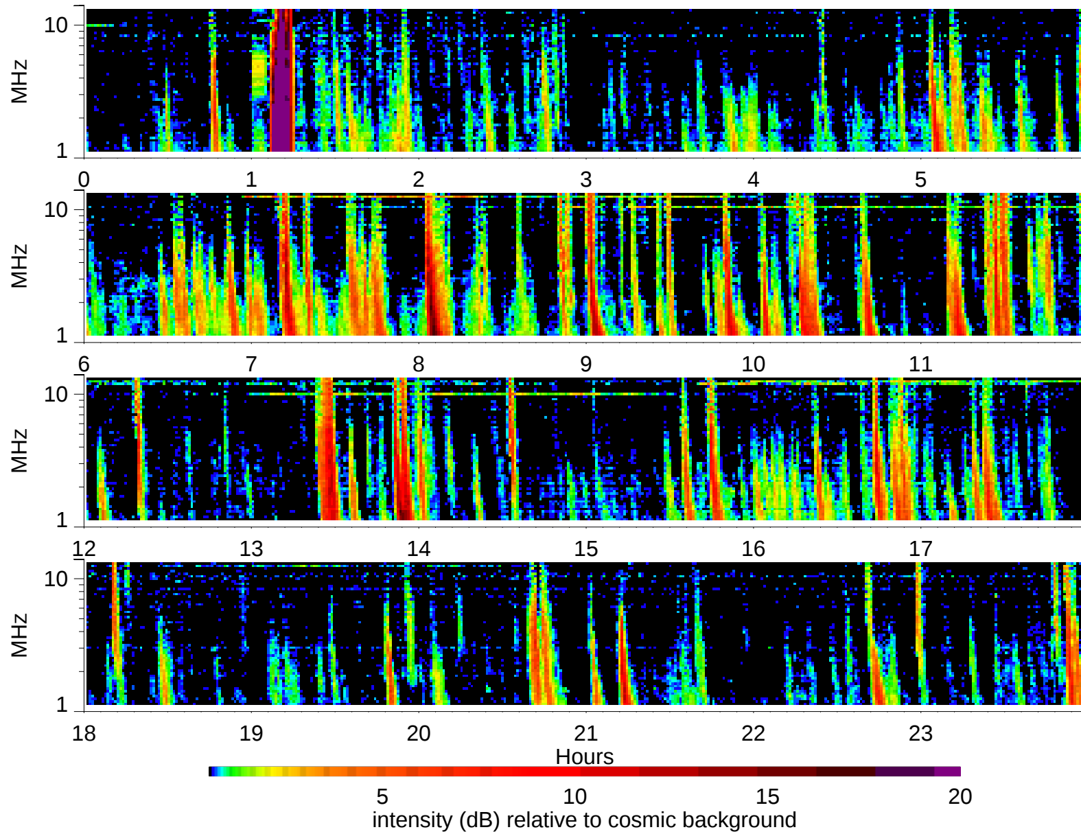
Wind Waves RAD2 receiver: 2003/4/12
