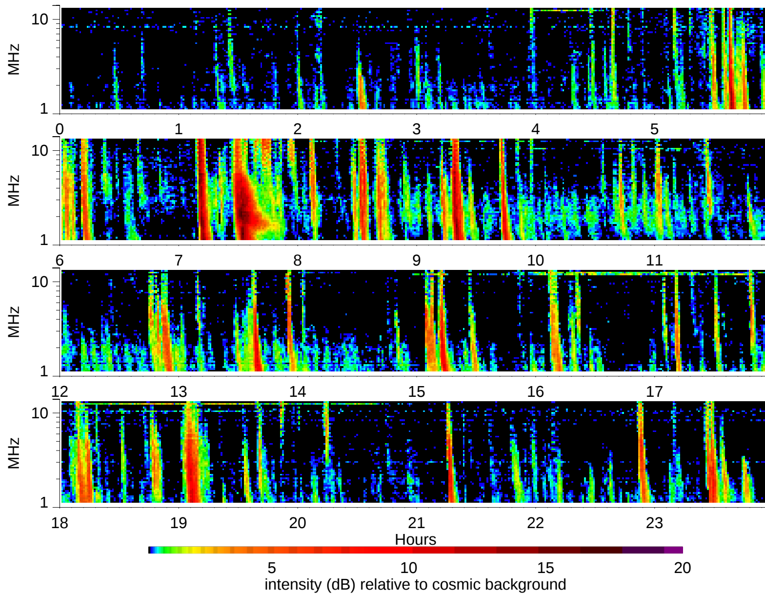
Wind Waves RAD2 receiver: 2003/4/11
