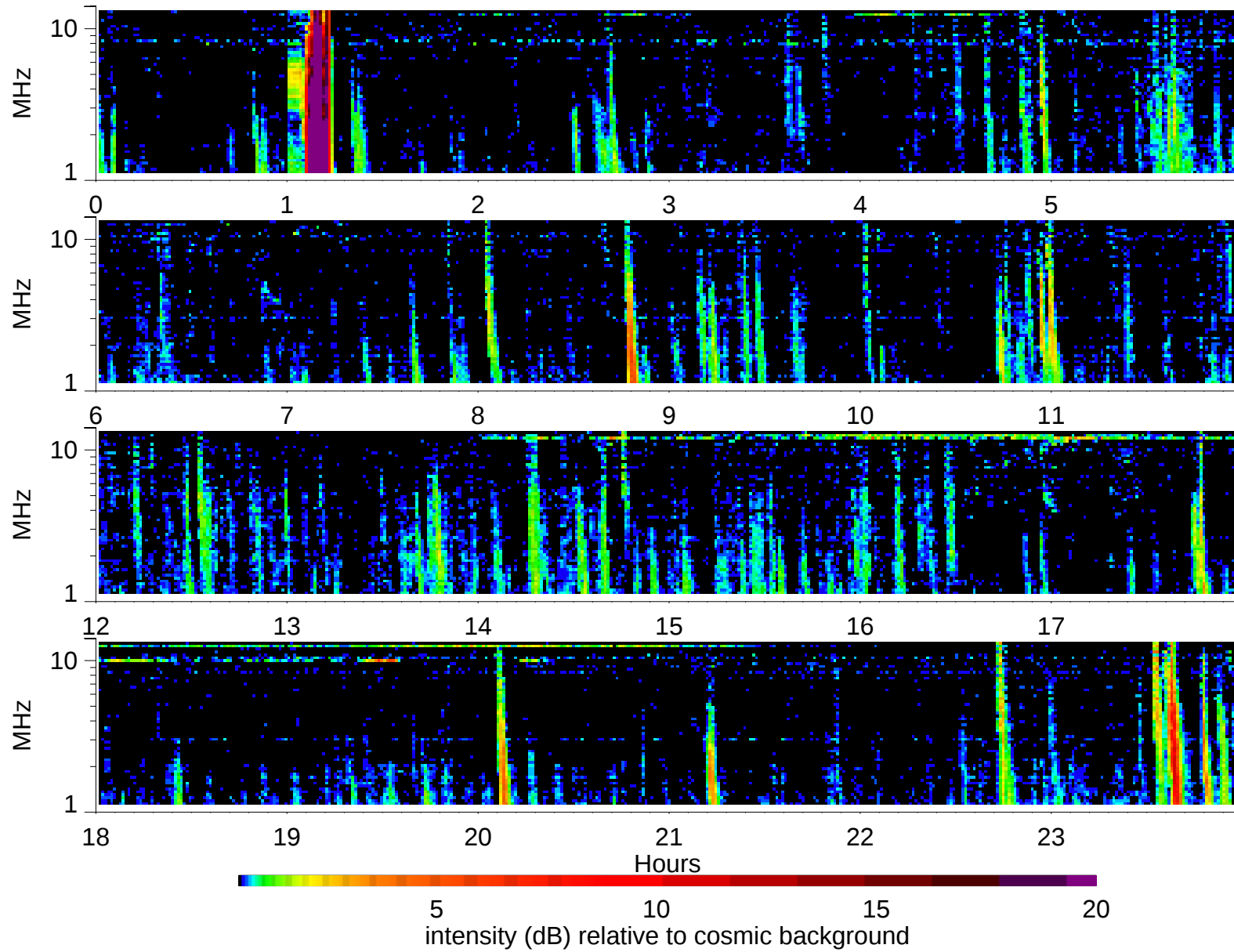
Wind Waves RAD2 receiver: 2003/4/10
