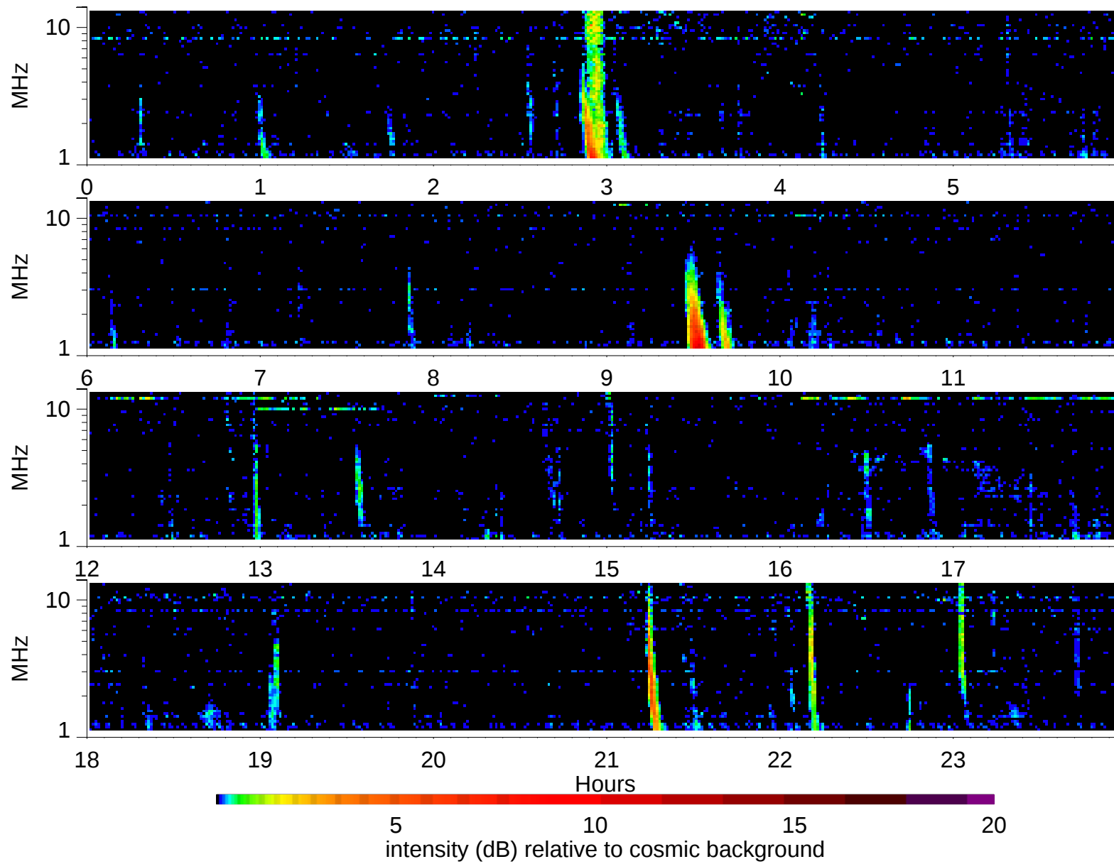
Wind Waves RAD2 receiver: 2003/4/7
