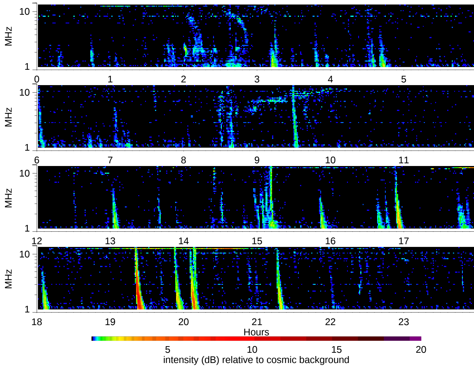
Wind Waves RAD2 receiver: 2003/4/5
