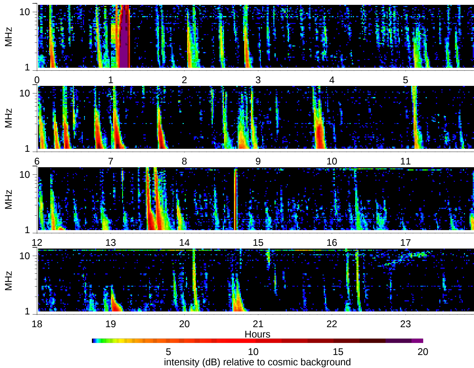
Wind Waves RAD2 receiver: 2003/4/4
